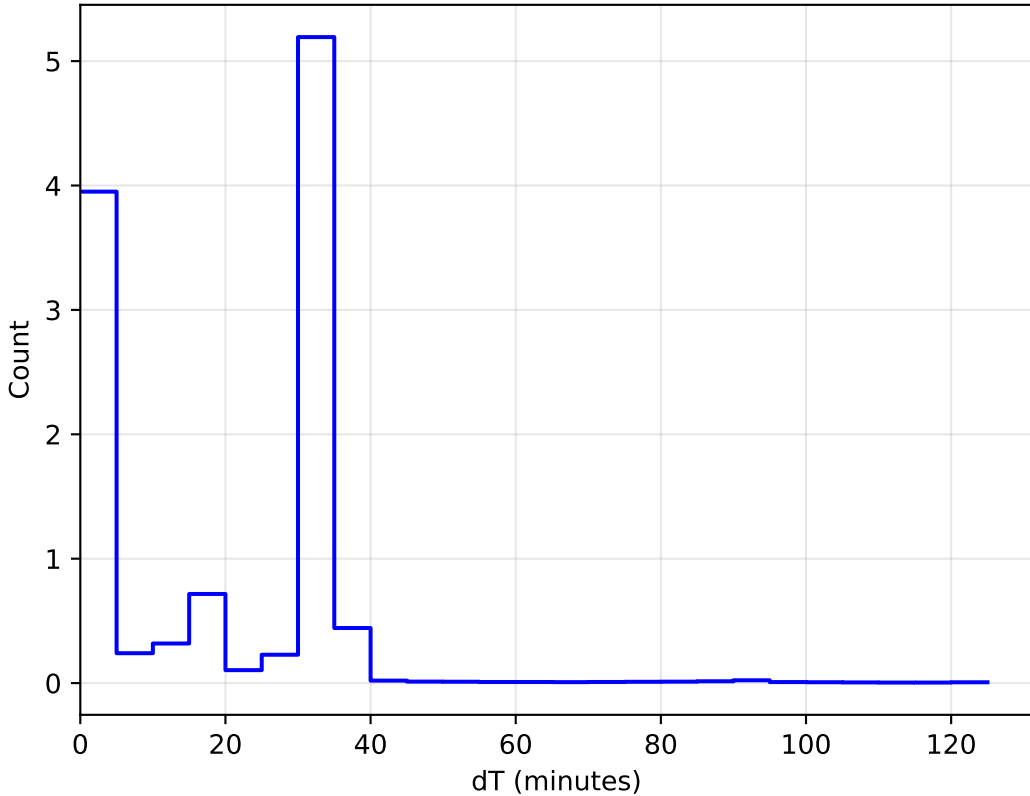
too_elab_r64_d3_giz_v3.4_10yrs WFD: DeltaT Histogram
