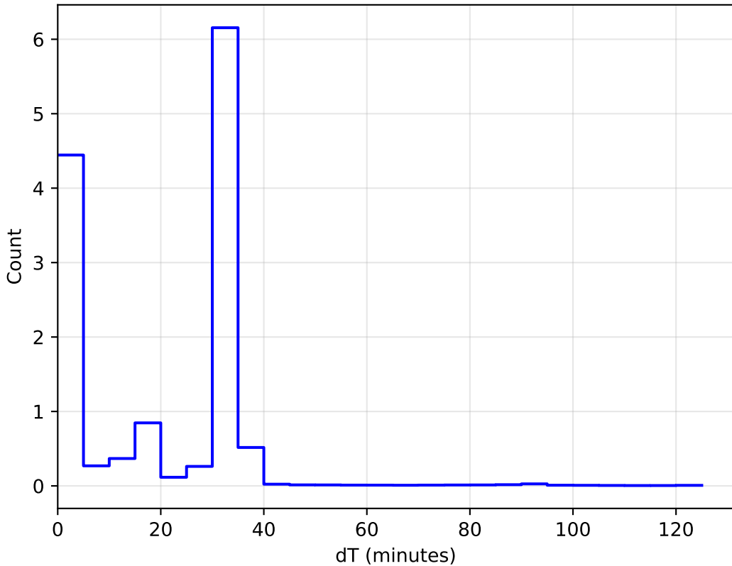
too_elab_r64_d3_giz_v3.4_10yrs All sky: DeltaT Histogram 1e6
