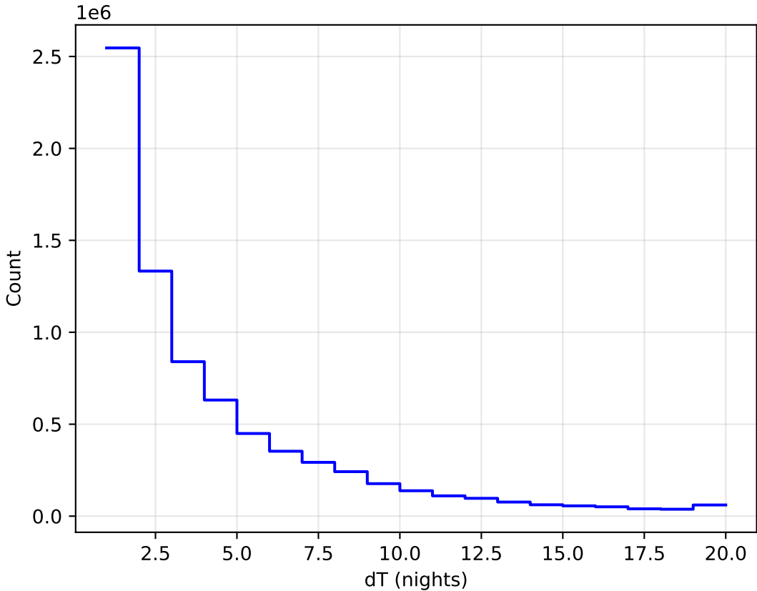
too_elab_r64_d3_giz_v3.4_10yrs WFD all bands: DeltaNight Histogram
