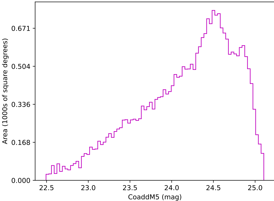
too_elab_r64_d3_giz_v3.4_10yrs Yr 3-4 z band: CoaddM5
