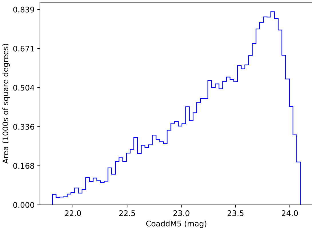
too_elab_r64_d3_giz_v3.4_10yrs Yr 3-4 y band: CoaddM5
