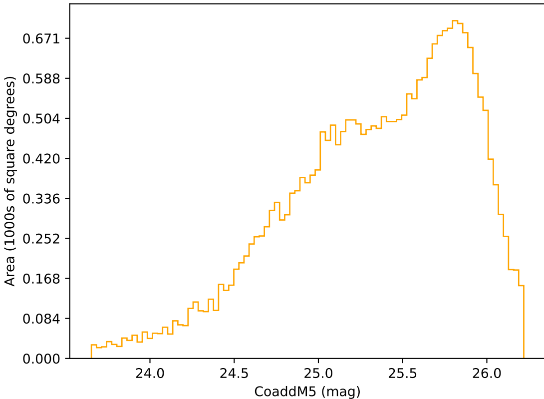
too_elab_r64_d3_giz_v3.4_10yrs Yr 3-4 r band: CoaddM5
