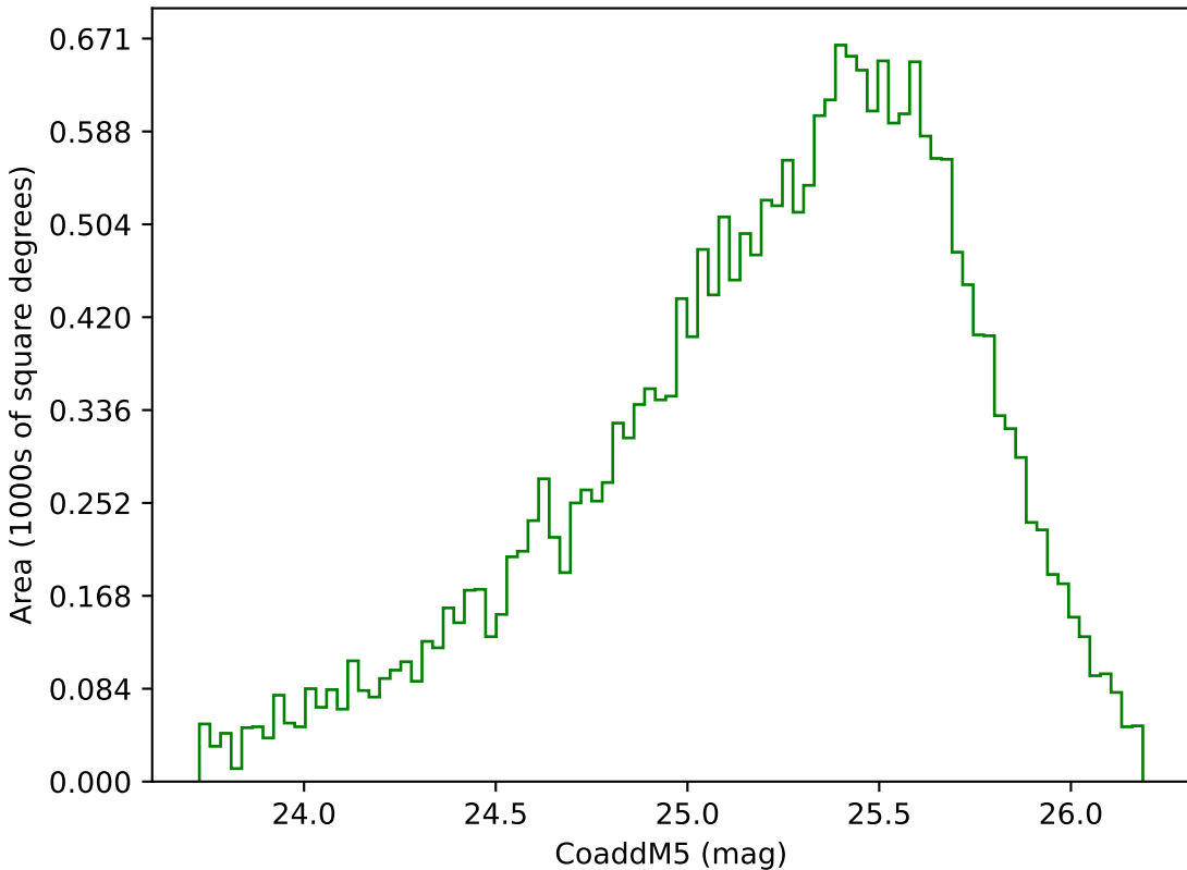
too_elab_r64_d3_giz_v3.4_10yrs Yr 3-4 g band: CoaddM5
