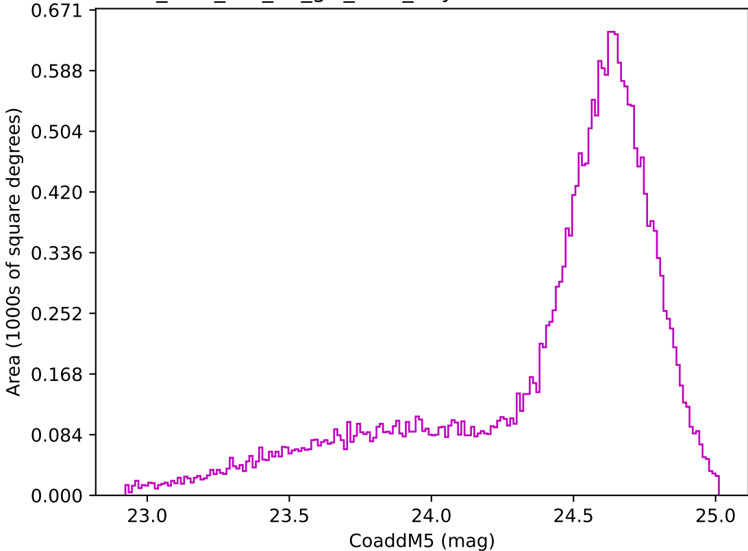
too_elab_r64_d3_giz_v3.4_10yrs Yr 1 z band: CoaddM5
