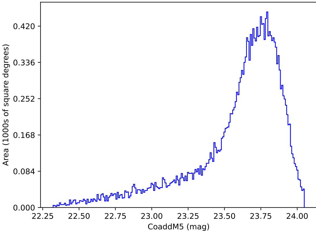
too_elab_r64_d3_giz_v3.4_10yrs Yr 1 y band: CoaddM5
