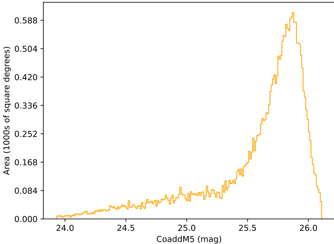
too_elab_r64_d3_giz_v3.4_10yrs Yr 1 r band: CoaddM5
