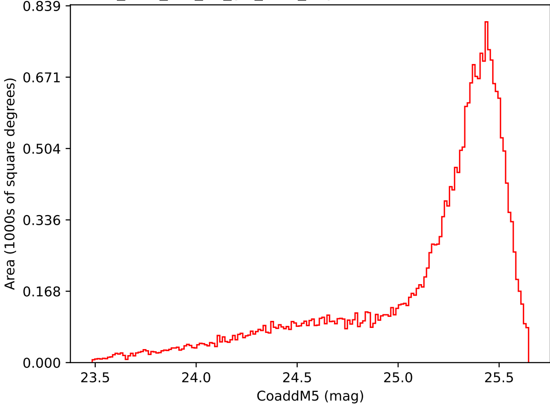
too_elab_r64_d3_giz_v3.4_10yrs Yr 1 i band: CoaddM5
