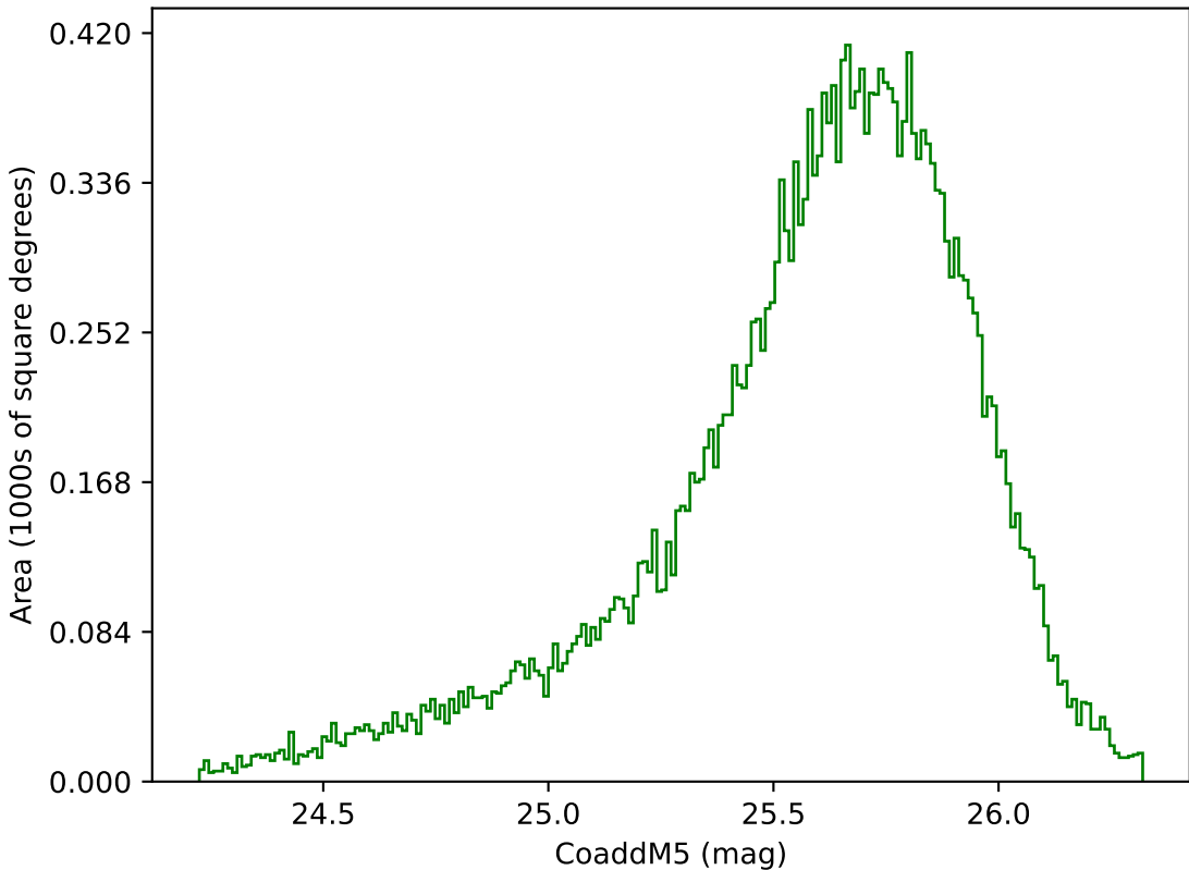
too_elab_r64_d3_giz_v3.4_10yrs Yr 1 g band: CoaddM5
