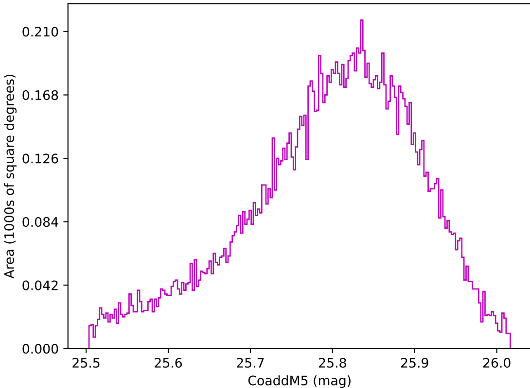
too_elab_r64_d3_giz_v3.4_10yrs WFD z band: CoaddM5
