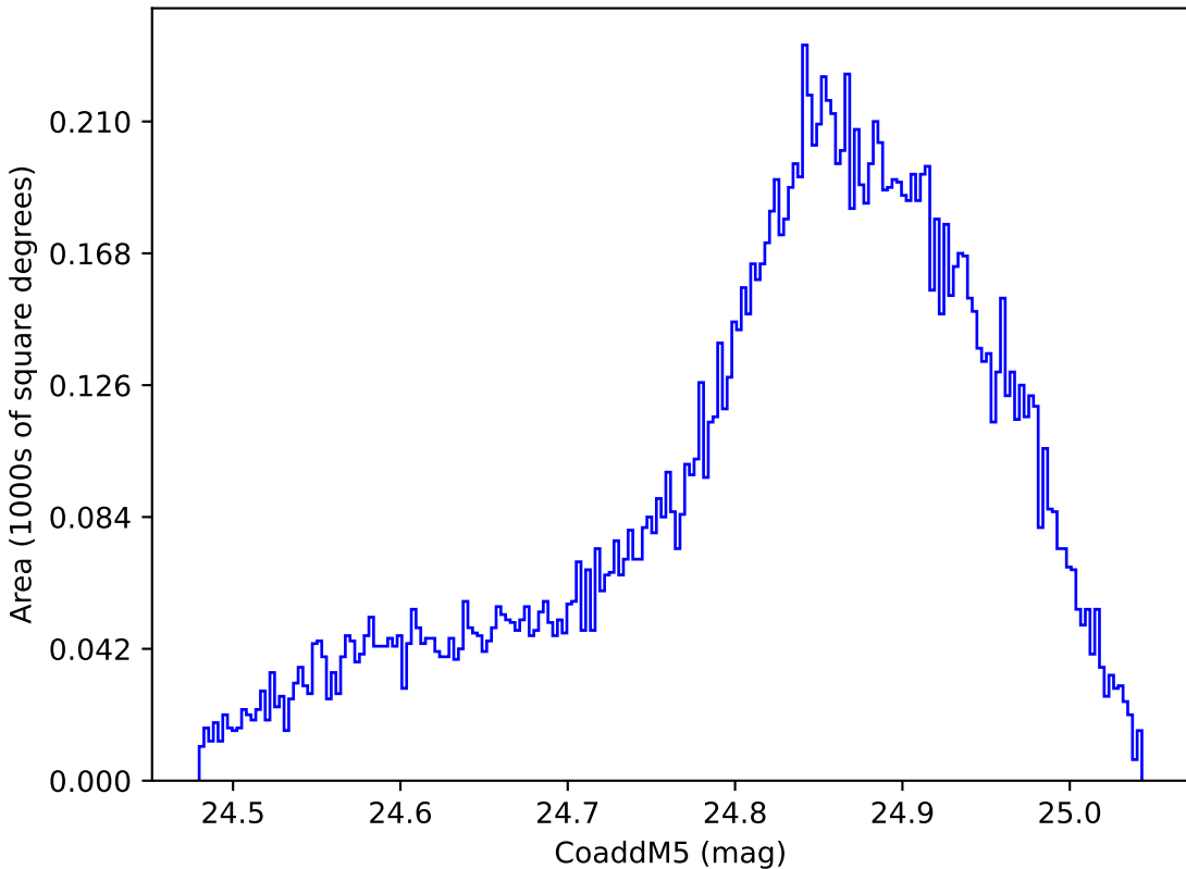
too_elab_r64_d3_giz_v3.4_10yrs WFD y band: CoaddM5
