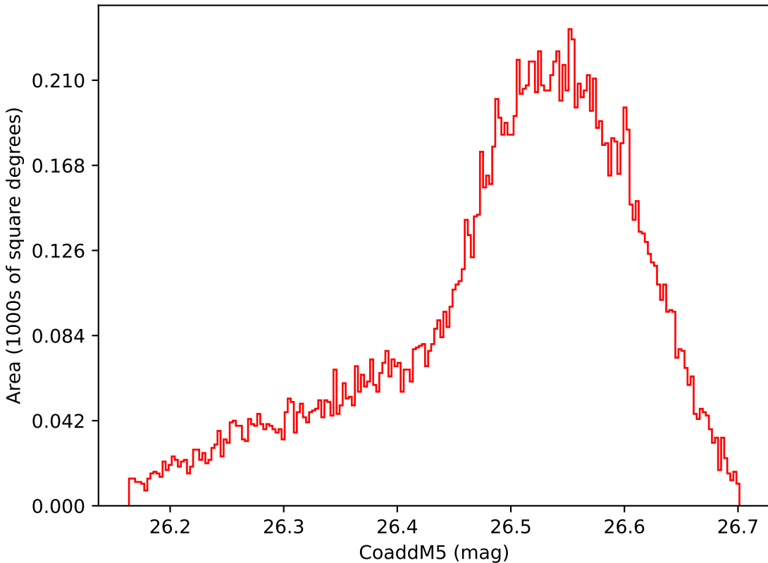
too_elab_r64_d3_giz_v3.4_10yrs WFD i band: CoaddM5
