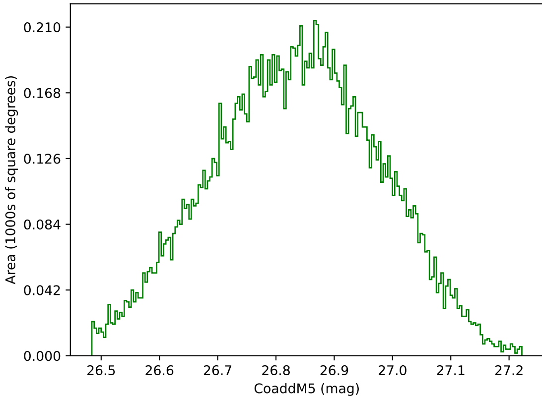
too_elab_r64_d3_giz_v3.4_10yrs WFD g band: CoaddM5
