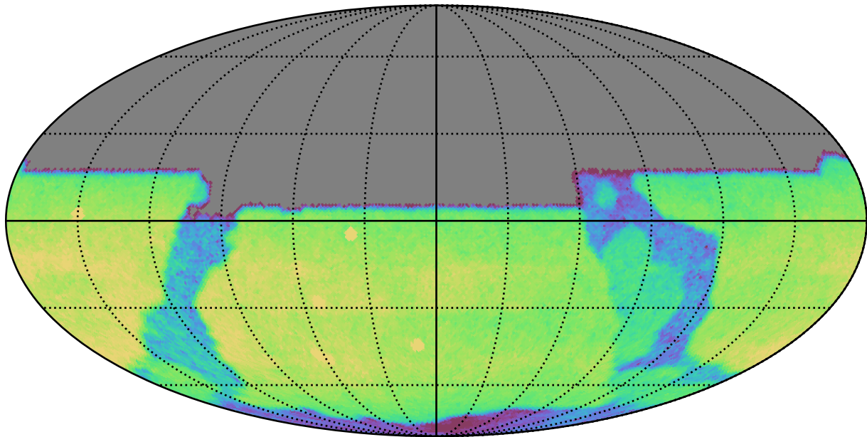
too_elab_r64_d3_giz_v3.4_10yrs All sky u band: CoaddM5
