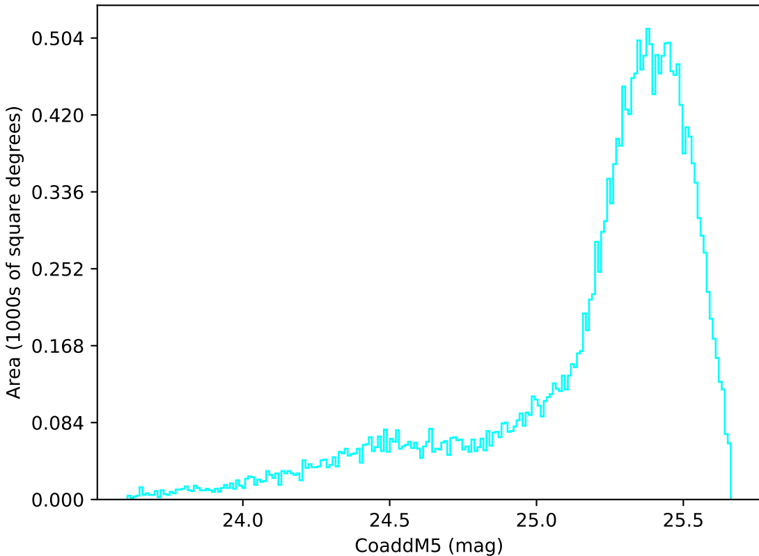
too_elab_r64_d3_giz_v3.4_10yrs All sky u band: CoaddM5
