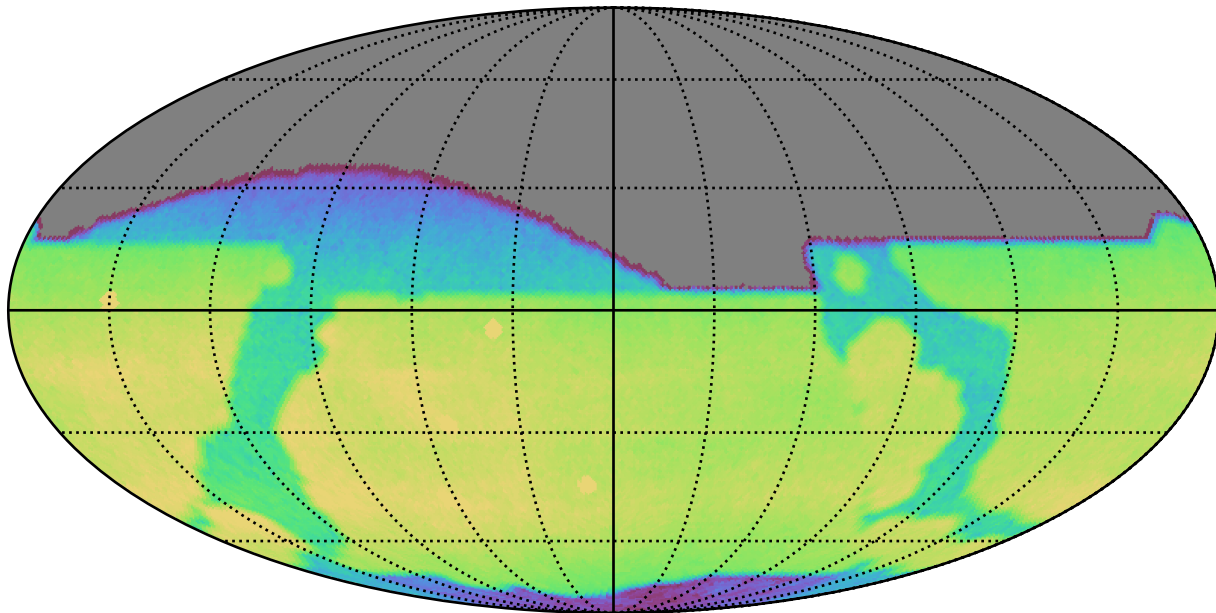
too_elab_r64_d3_giz_v3.4_10yrs All sky r band: CoaddM5
