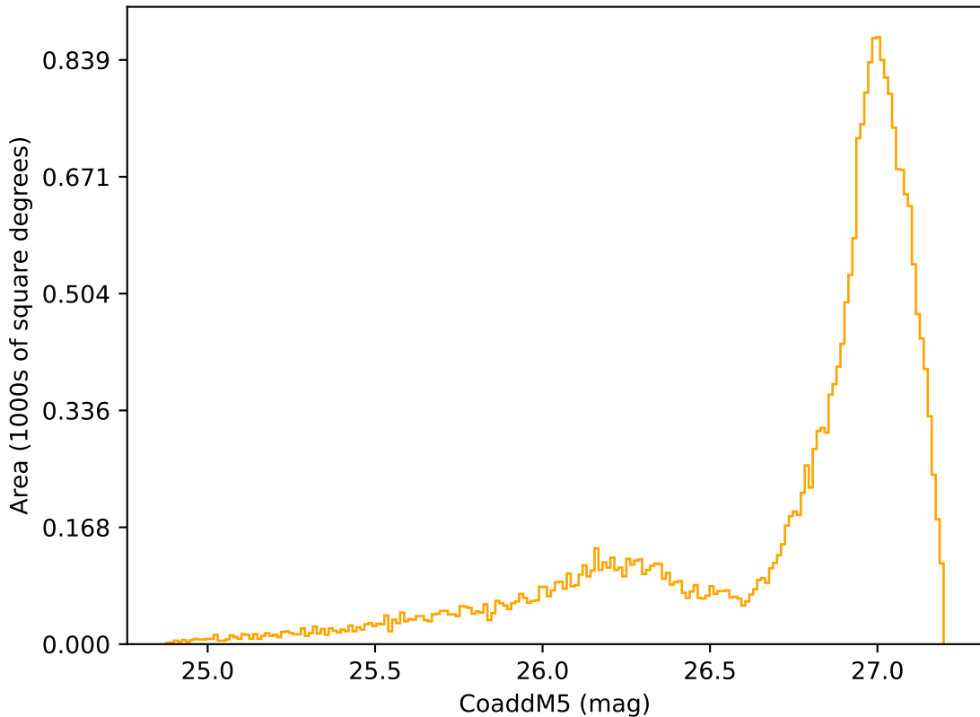
too_elab_r64_d3_giz_v3.4_10yrs All sky r band: CoaddM5
