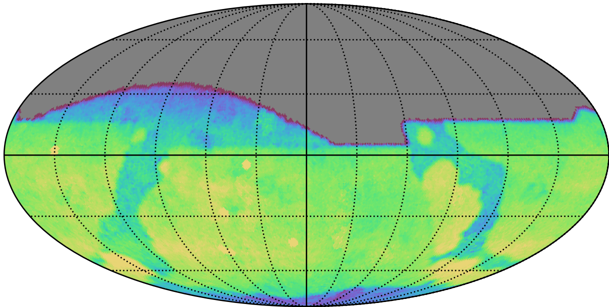
too_elab_r64_d3_giz_v3.4_10yrs All sky g band: CoaddM5
