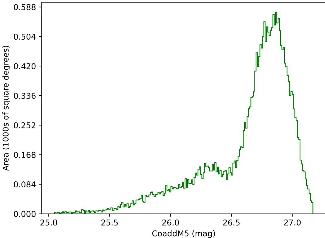
too_elab_r64_d3_giz_v3.4_10yrs All sky g band: CoaddM5
