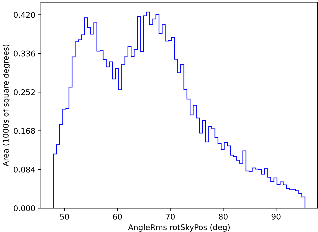
too_elab_r64_d3_giz_v3.4_10yrs WFD z band: AngleRms rotSkyPos
