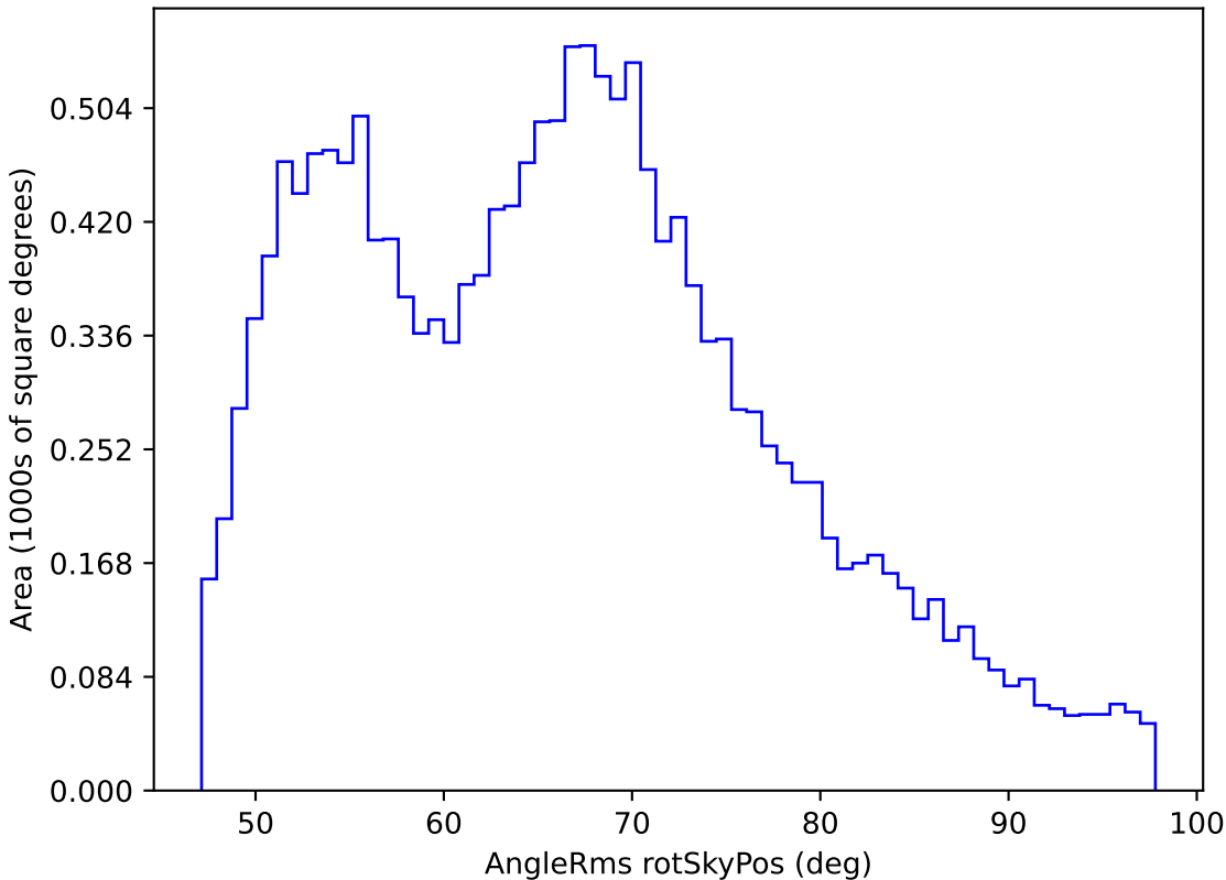
too_elab_r64_d3_giz_v3.4_10yrs WFD r band: AngleRms rotSkyPos
