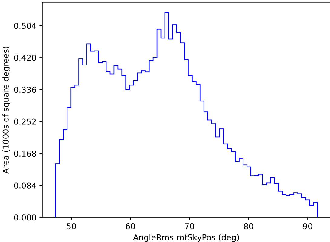
too_elab_r64_d3_giz_v3.4_10yrs WFD i band: AngleRms rotSkyPos
