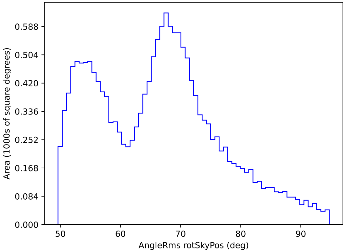
too_elab_r64_d3_giz_v3.4_10yrs WFD all bands: AngleRms rotSkyPos
