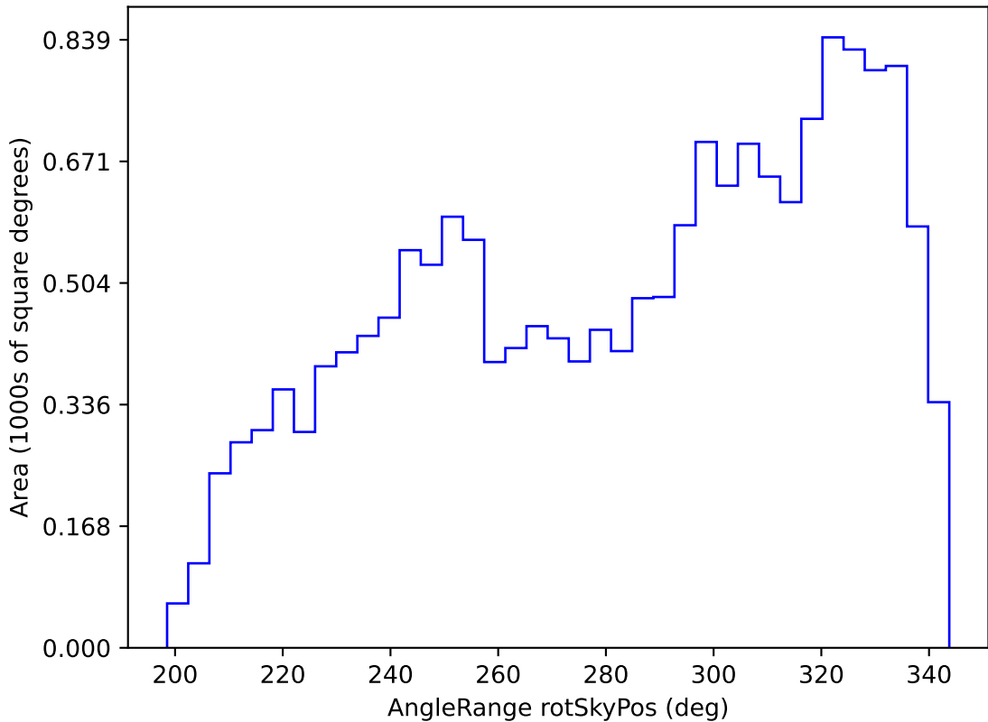
too_elab_r64_d3_giz_v3.4_10yrs WFD r band: AngleRange rotSkyPos
