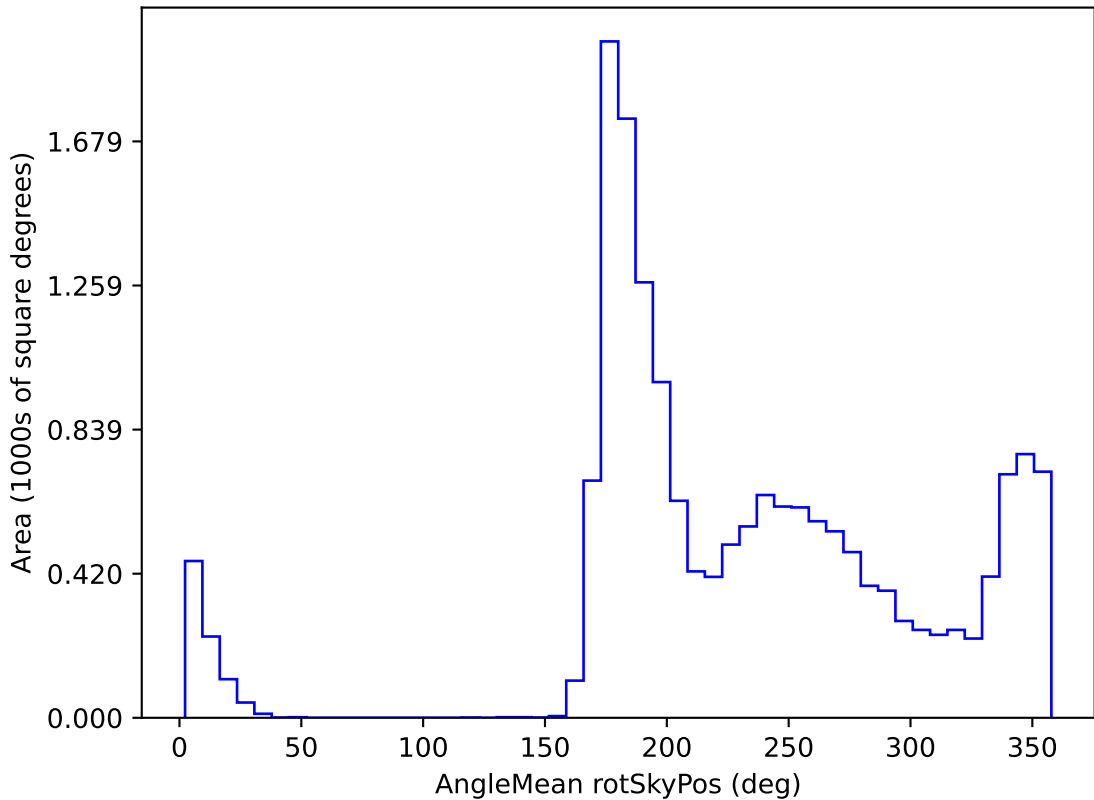
too_elab_r64_d3_giz_v3.4_10yrs WFD y band: AngleMean rotSkyPos
