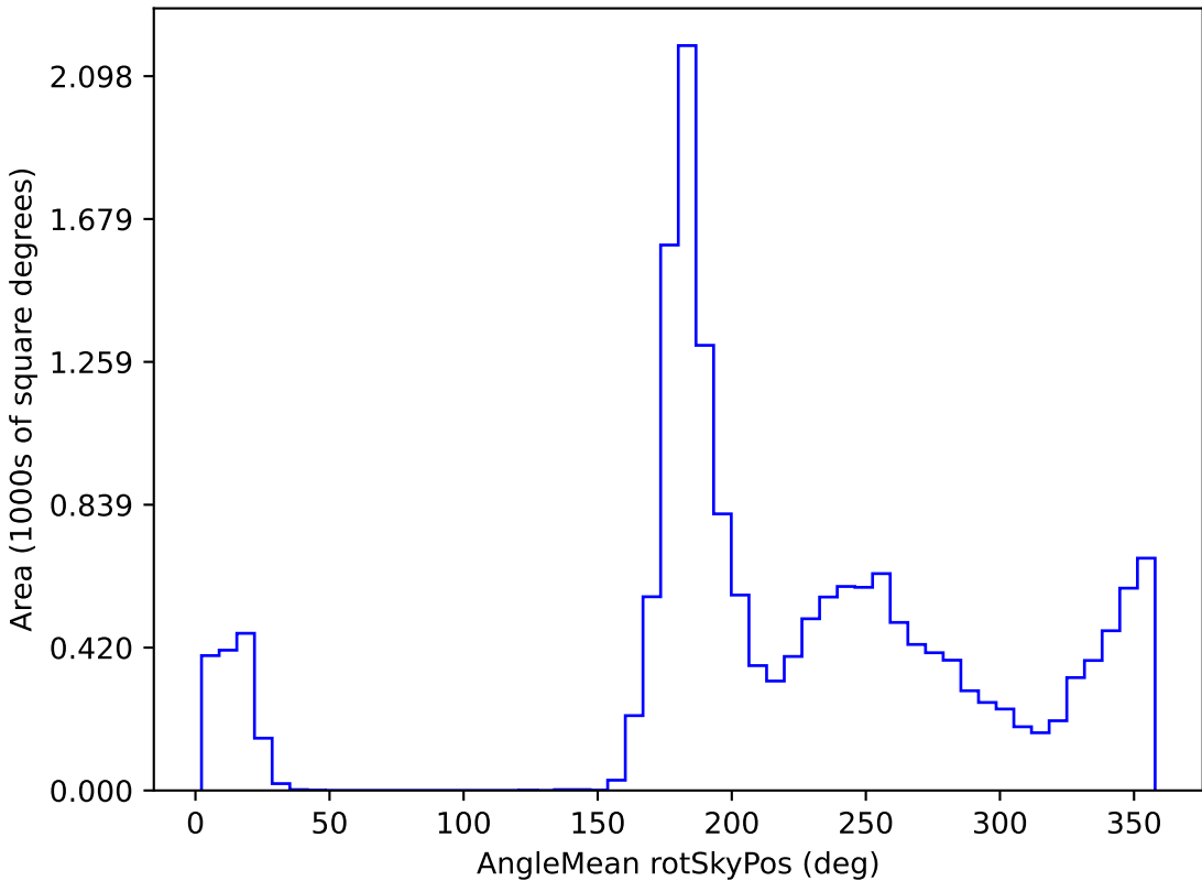
too_elab_r64_d3_giz_v3.4_10yrs WFD i band: AngleMean rotSkyPos
