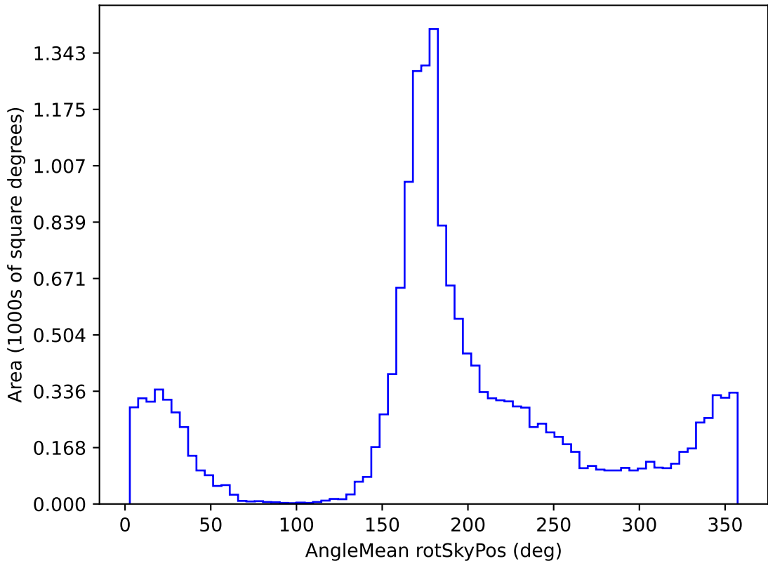
too_elab_r64_d3_giz_v3.4_10yrs WFD g band: AngleMean rotSkyPos
