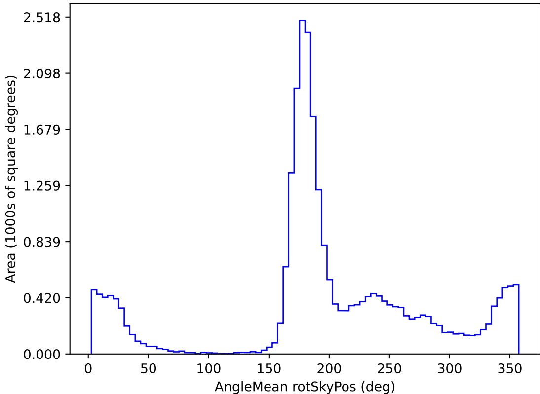
too_elab_r64_d3_giz_v3.4_10yrs All sky r band: AngleMean rotSkyPos
