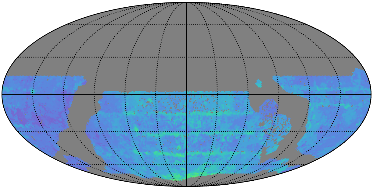
too_elab_r64_d3_giz_v3.4_10yrs WFD y band: 80thPercentile Season Length
