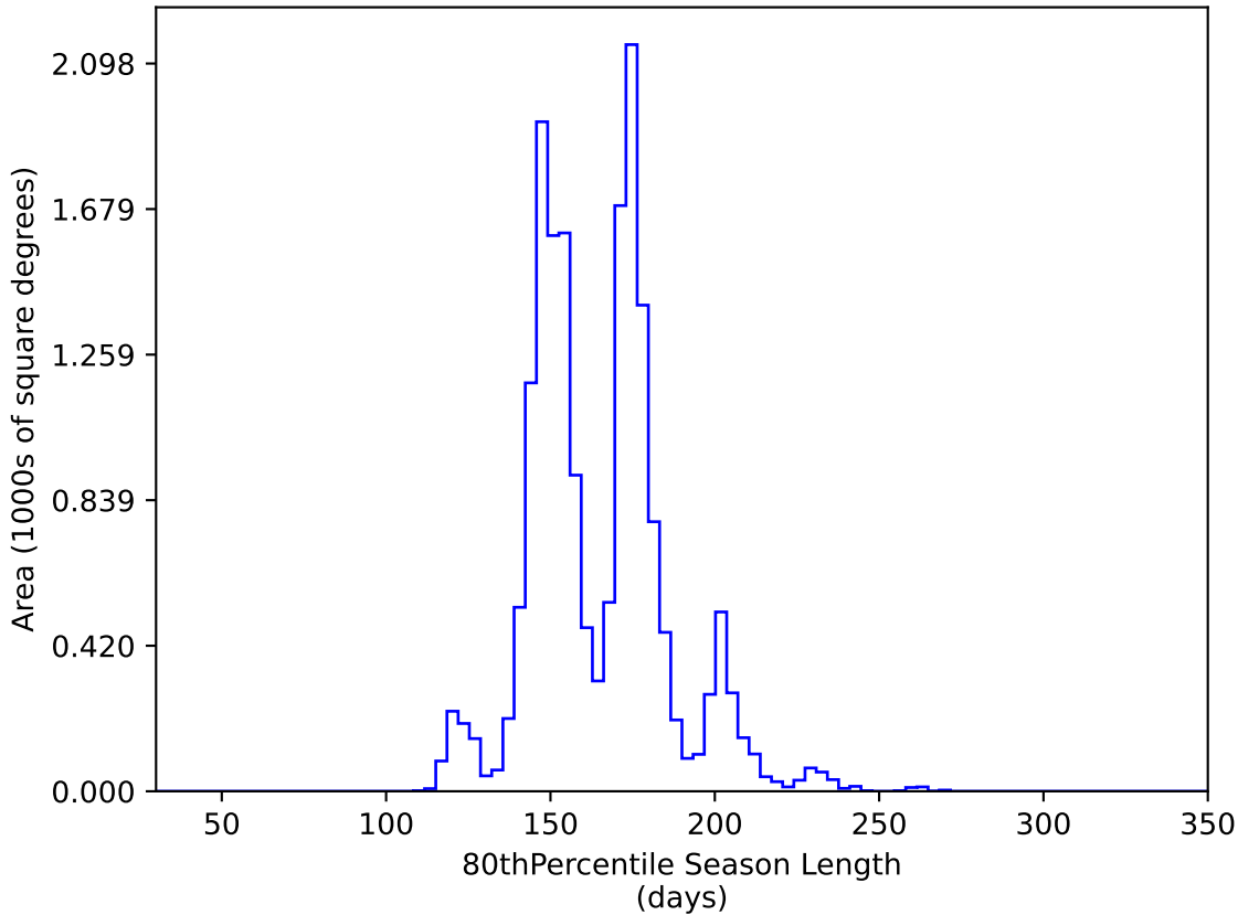
too_elab_r64_d3_giz_v3.4_10yrs WFD y band: 80thPercentile Season Length
