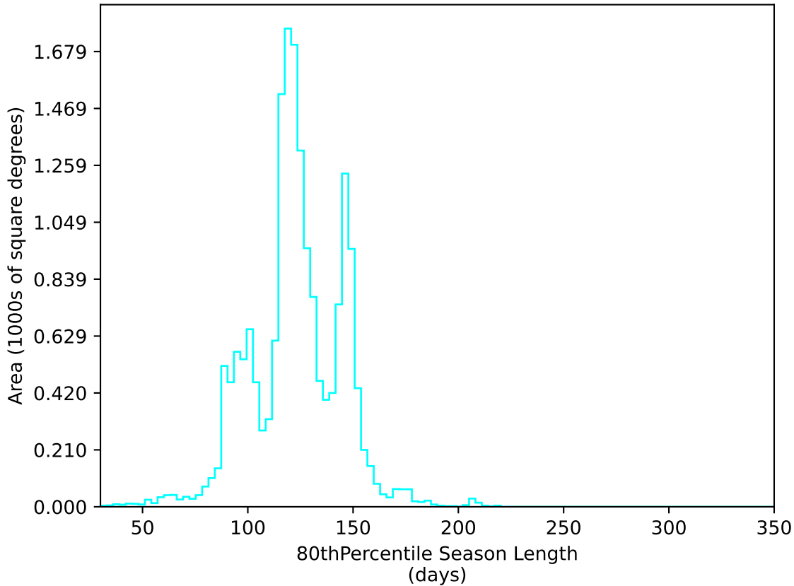
too_elab_r64_d3_giz_v3.4_10yrs WFD u band: 80thPercentile Season Length
