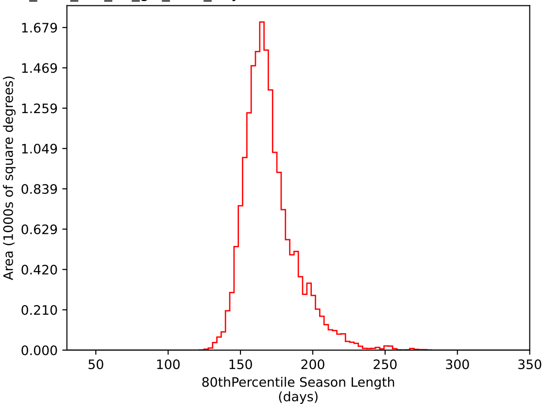
too_elab_r64_d3_giz_v3.4_10yrs WFD i band: 80thPercentile Season Length
