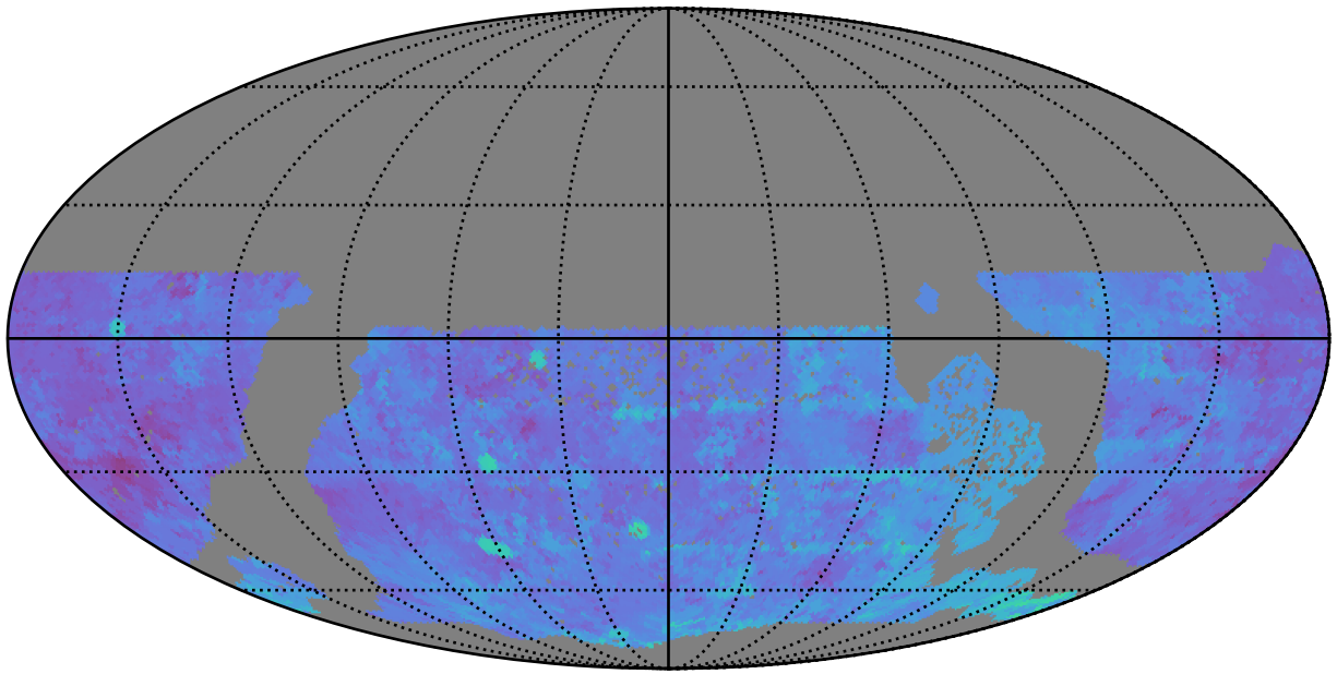
too_elab_r64_d3_giz_v3.4_10yrs WFD g band: 80thPercentile Season Length
