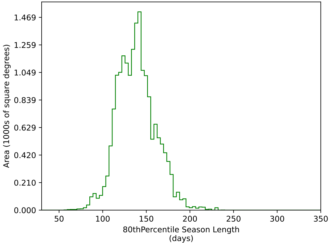
too_elab_r64_d3_giz_v3.4_10yrs WFD g band: 80thPercentile Season Length
