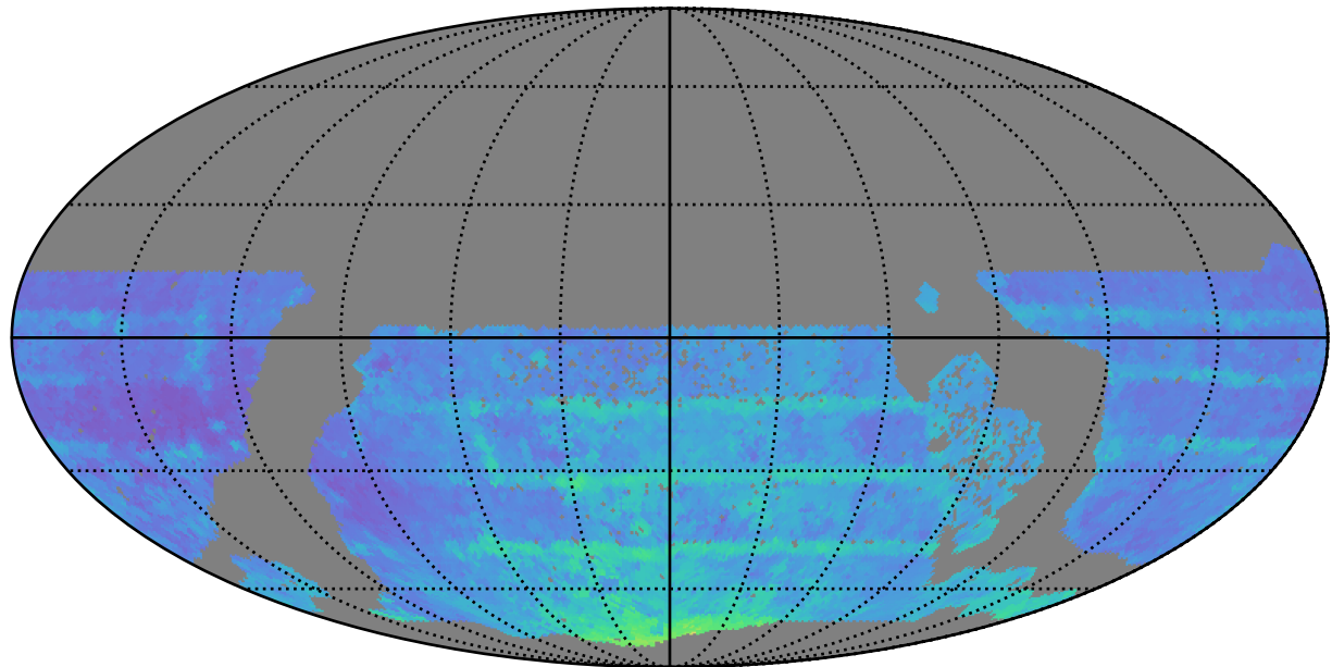
too_elab_r64_d3_giz_v3.4_10yrs WFD all bands: 80thPercentile Season Length
