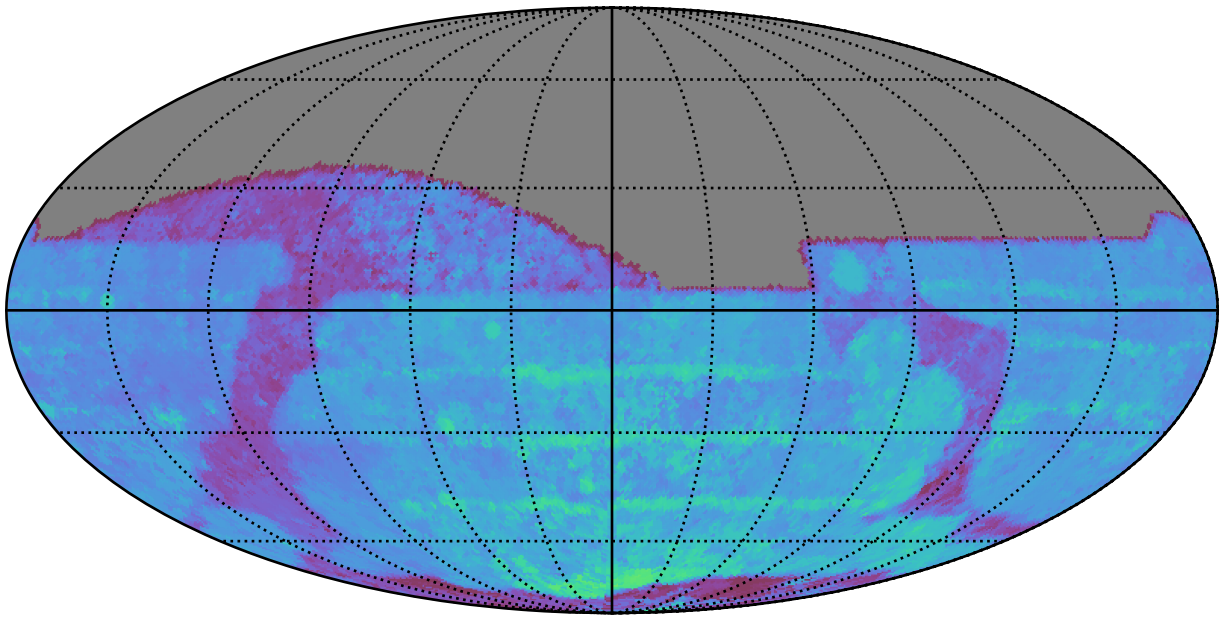
too_elab_r64_d3_giz_v3.4_10yrs All sky z band: 80thPercentile Season Length
