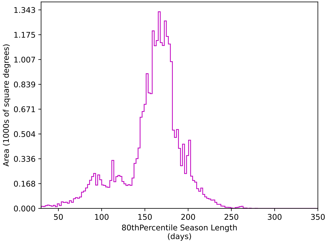
too_elab_r64_d3_giz_v3.4_10yrs All sky z band: 80thPercentile Season Length
