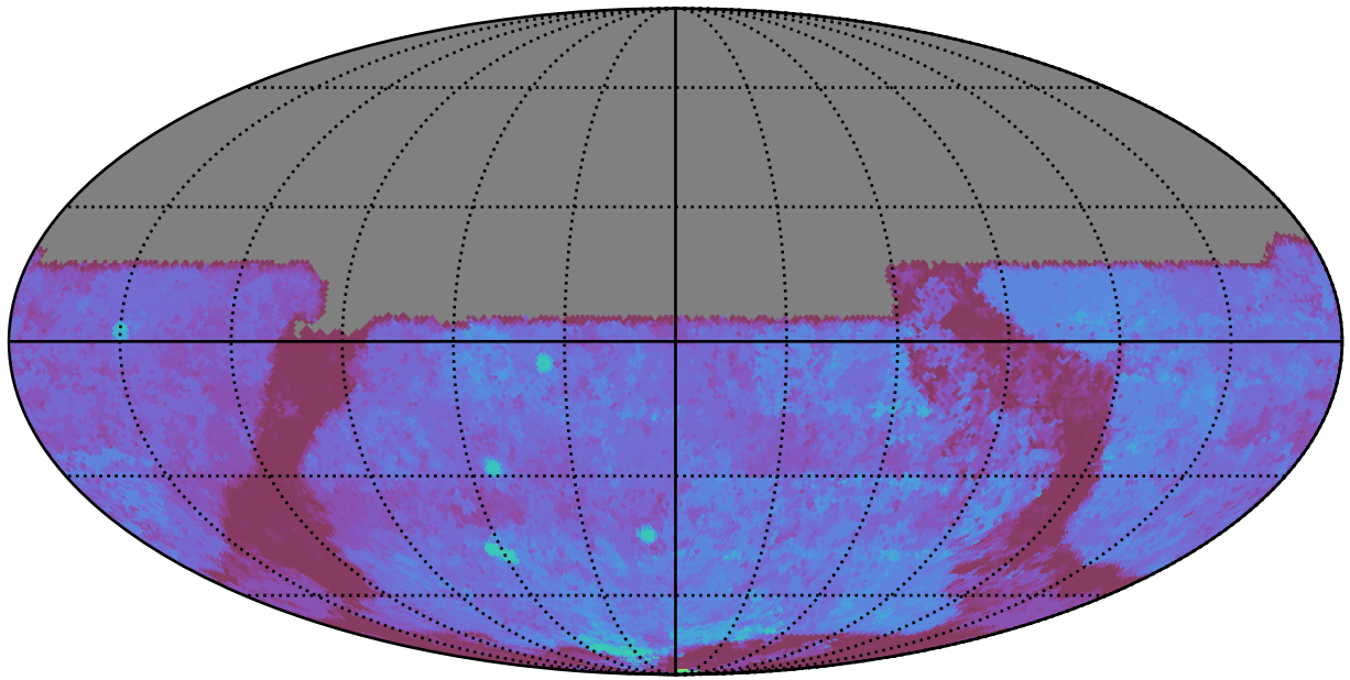
too_elab_r64_d3_giz_v3.4_10yrs All sky u band: 80thPercentile Season Length
