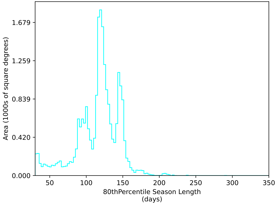
too_elab_r64_d3_giz_v3.4_10yrs All sky u band: 80thPercentile Season Length
