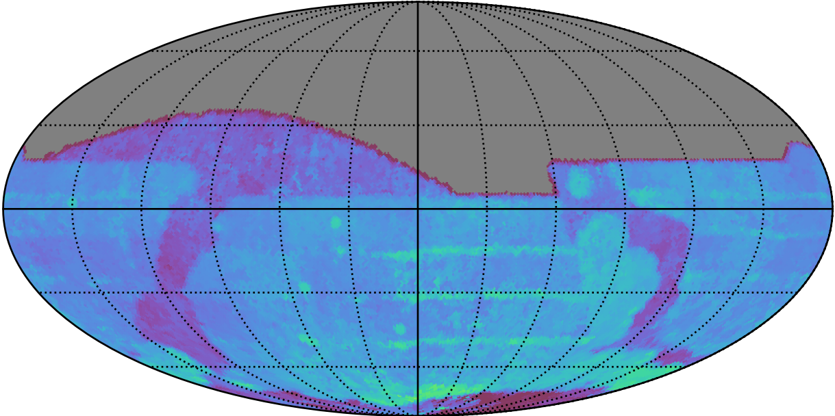
too_elab_r64_d3_giz_v3.4_10yrs All sky r band: 80thPercentile Season Length
