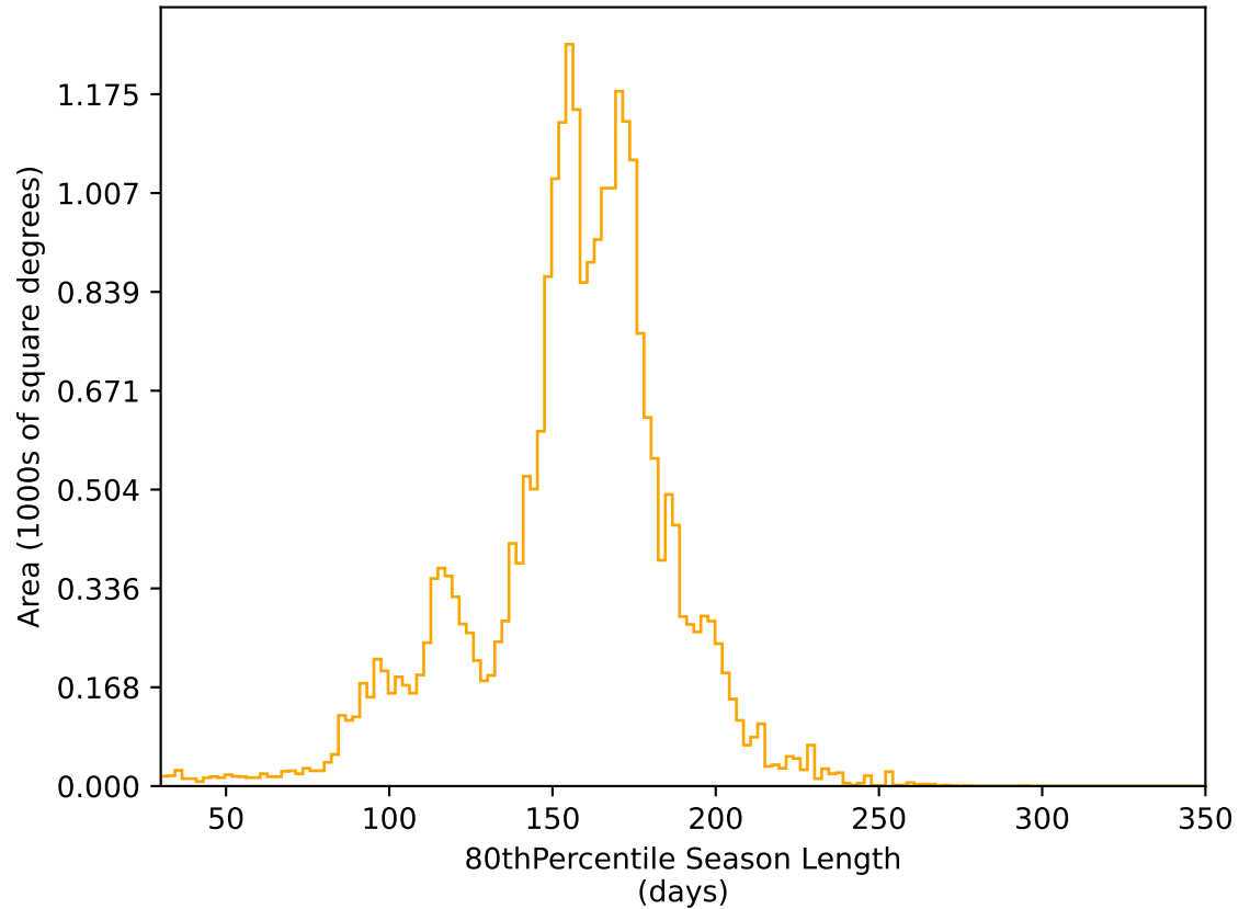
too_elab_r64_d3_giz_v3.4_10yrs All sky r band: 80thPercentile Season Length
