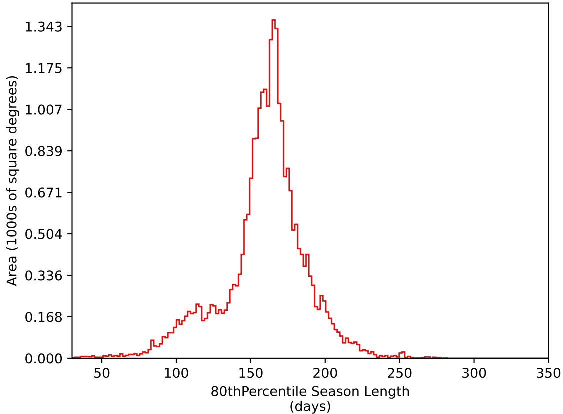
too_elab_r64_d3_giz_v3.4_10yrs All sky i band: 80thPercentile Season Length
