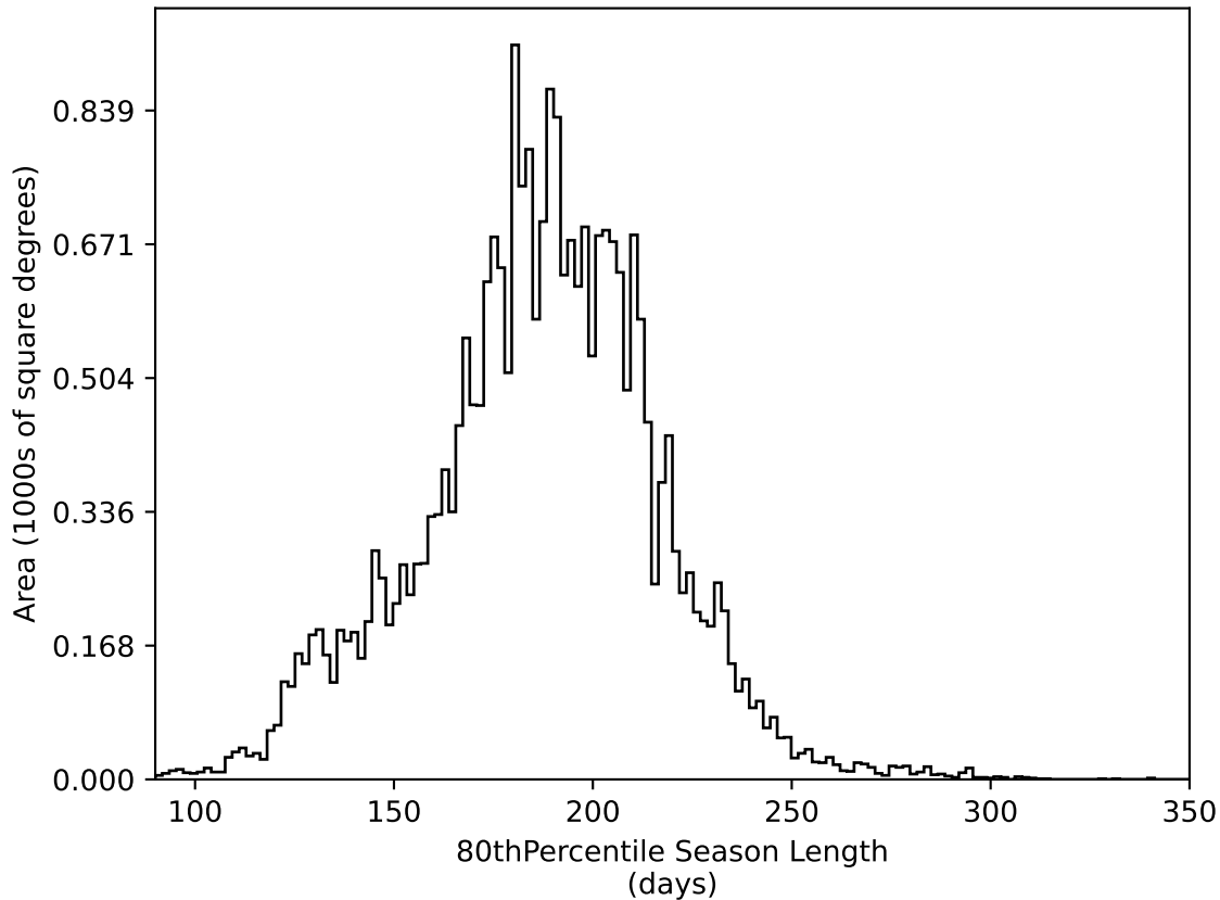
too_elab_r64_d3_giz_v3.4_10yrs All sky all bands: 80thPercentile Season Length
