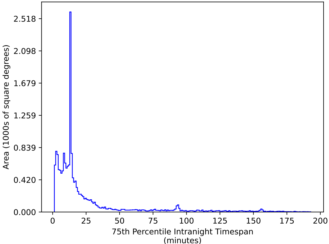
too_elab_r64_d3_giz_v3.4_10yrs WFD z band: 75th Percentile Intranight Timespan
