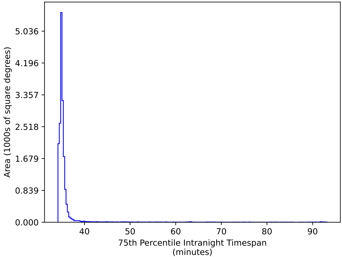
too_elab_r64_d3_giz_v3.4_10yrs WFD ri bands: 75th Percentile Intranight Timespan
