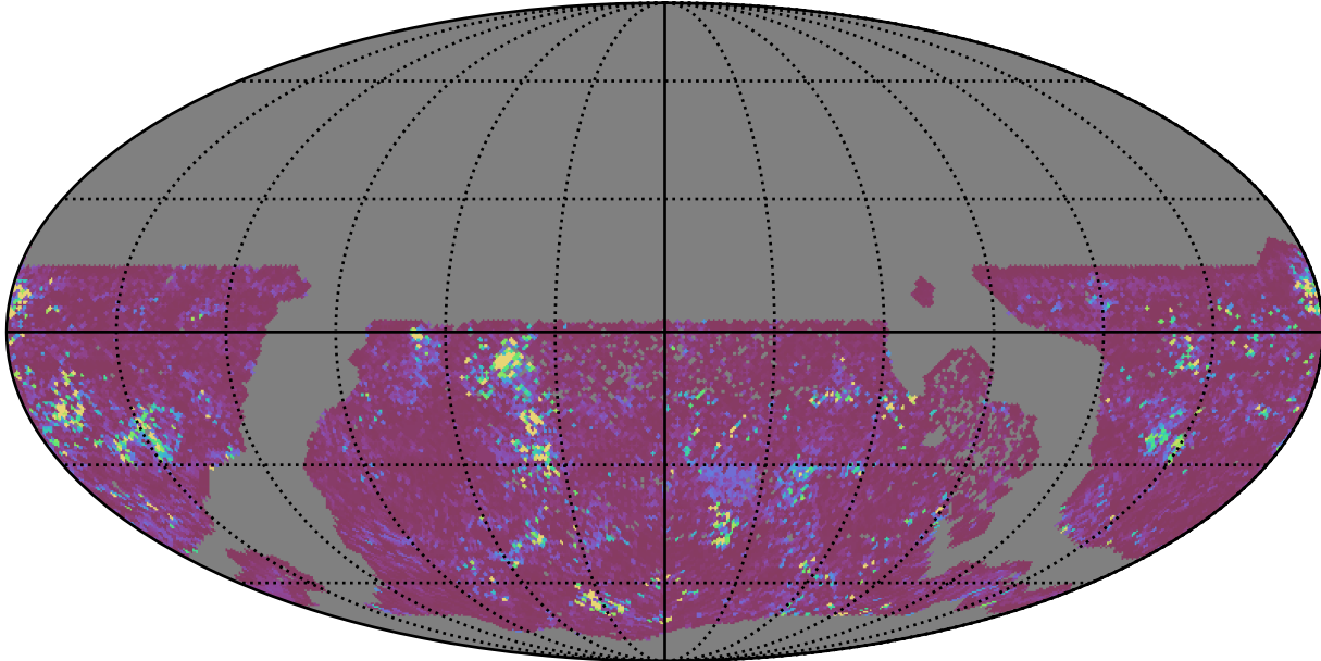
too_elab_r64_d3_giz_v3.4_10yrs WFD g band: 75th Percentile Intranight Timespan
