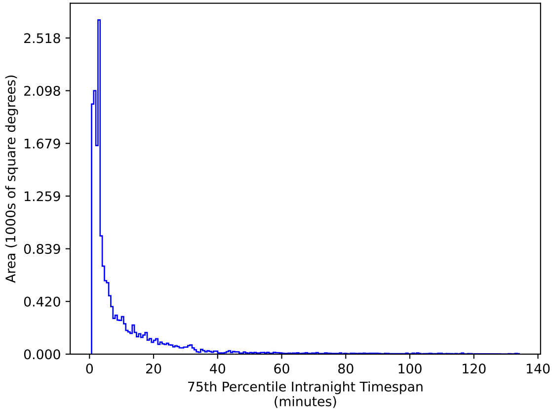
too_elab_r64_d3_giz_v3.4_10yrs WFD g band: 75th Percentile Intranight Timespan
